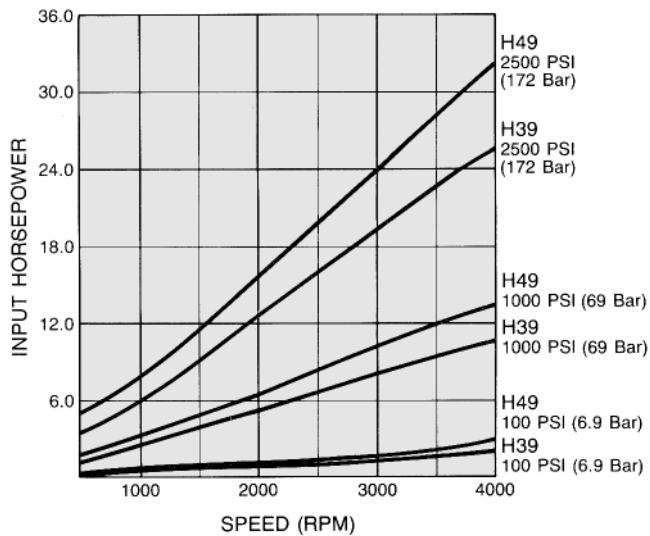
H39/H49 Horsepower/Speed
